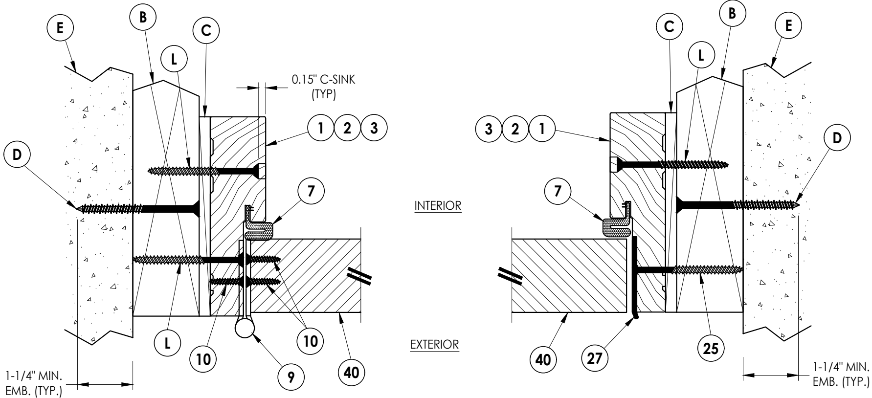
2 3 HORIZONTAL CROSS SECTION Outswing shown (Inswing similar)
